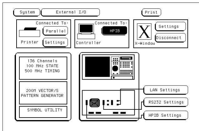
HP-IB Connection
